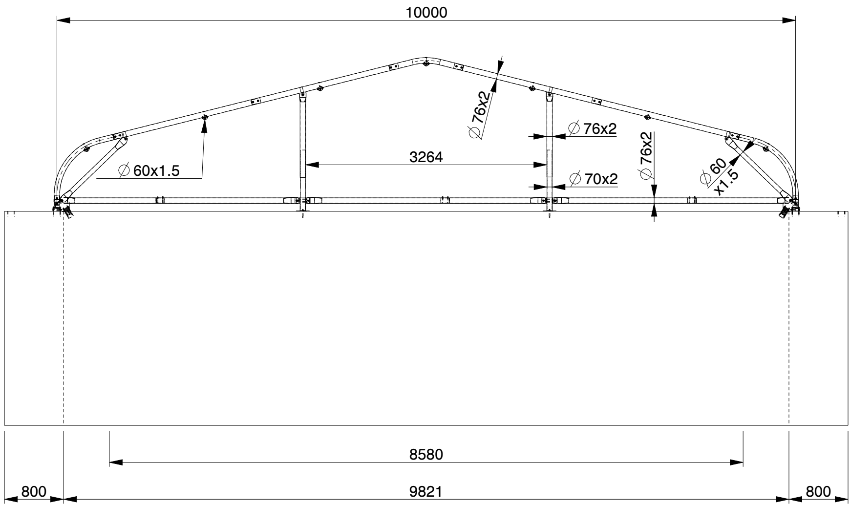
Rear view
