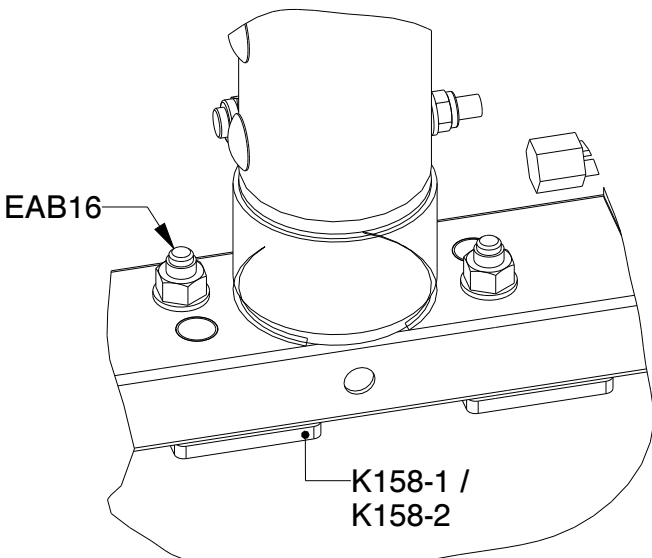
DETAIL F SCALE 1:4
