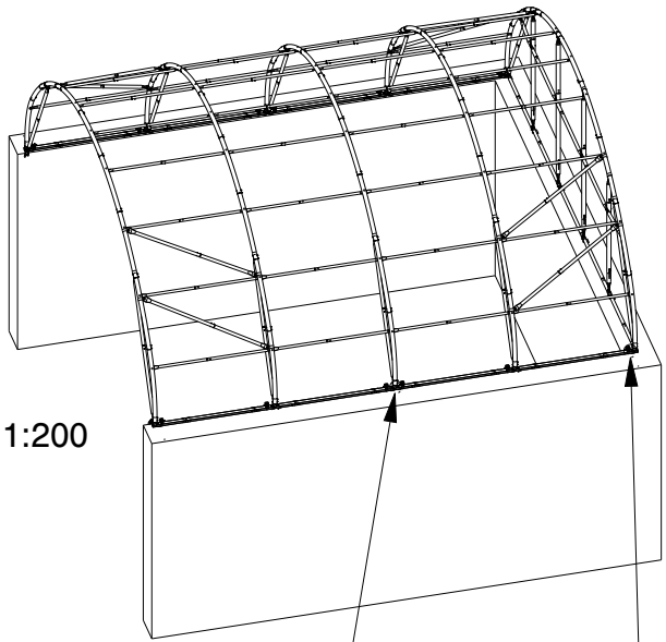
SEE DETAIL F SEE DETAIL D
