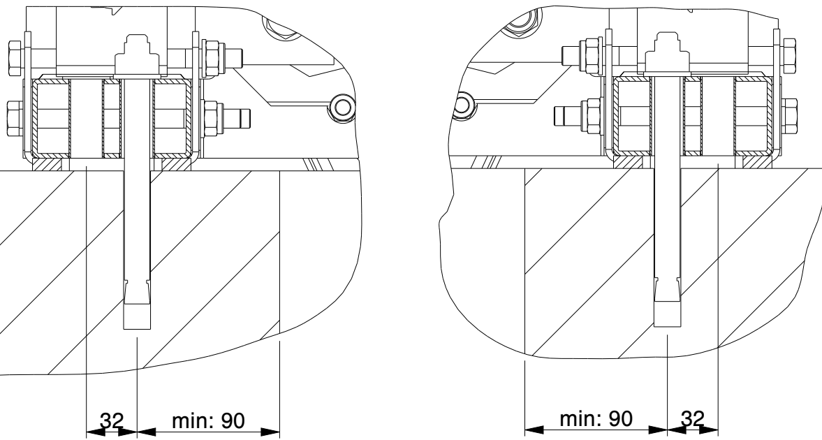
DETAIL C SCALE 3:10
