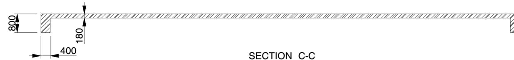
SECTION C-C
