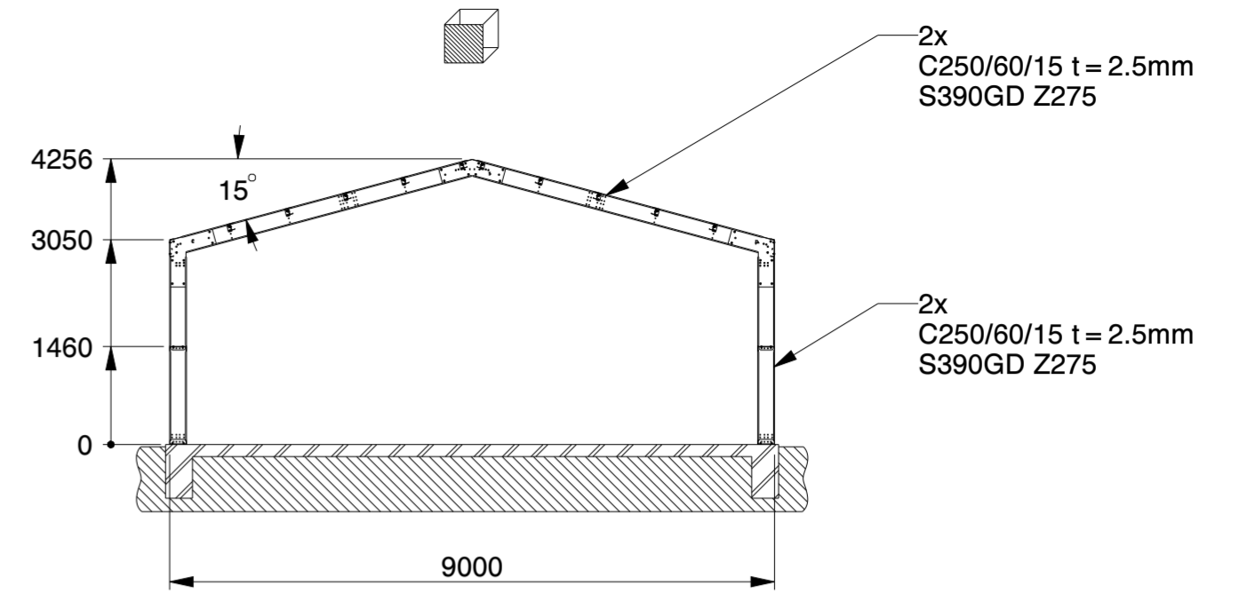
SECTION B-B
