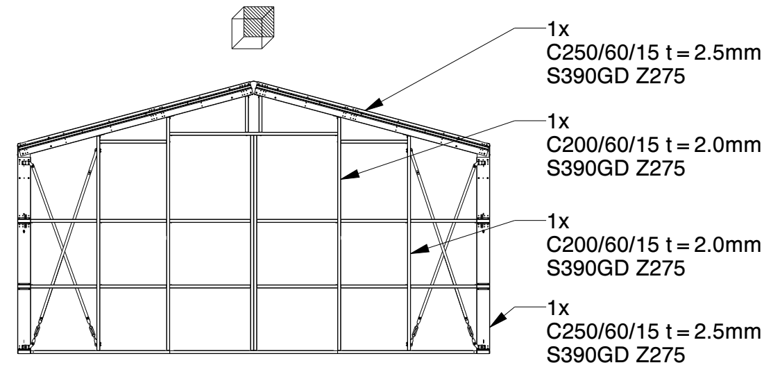
BACK WALL
