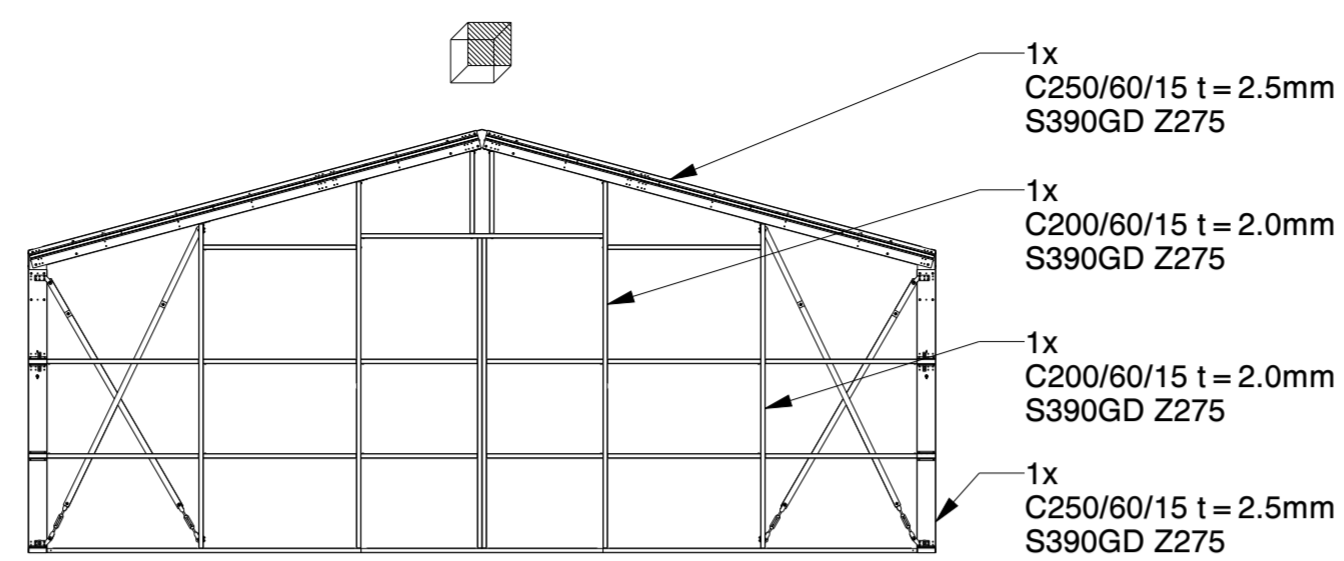
BACK WALL
