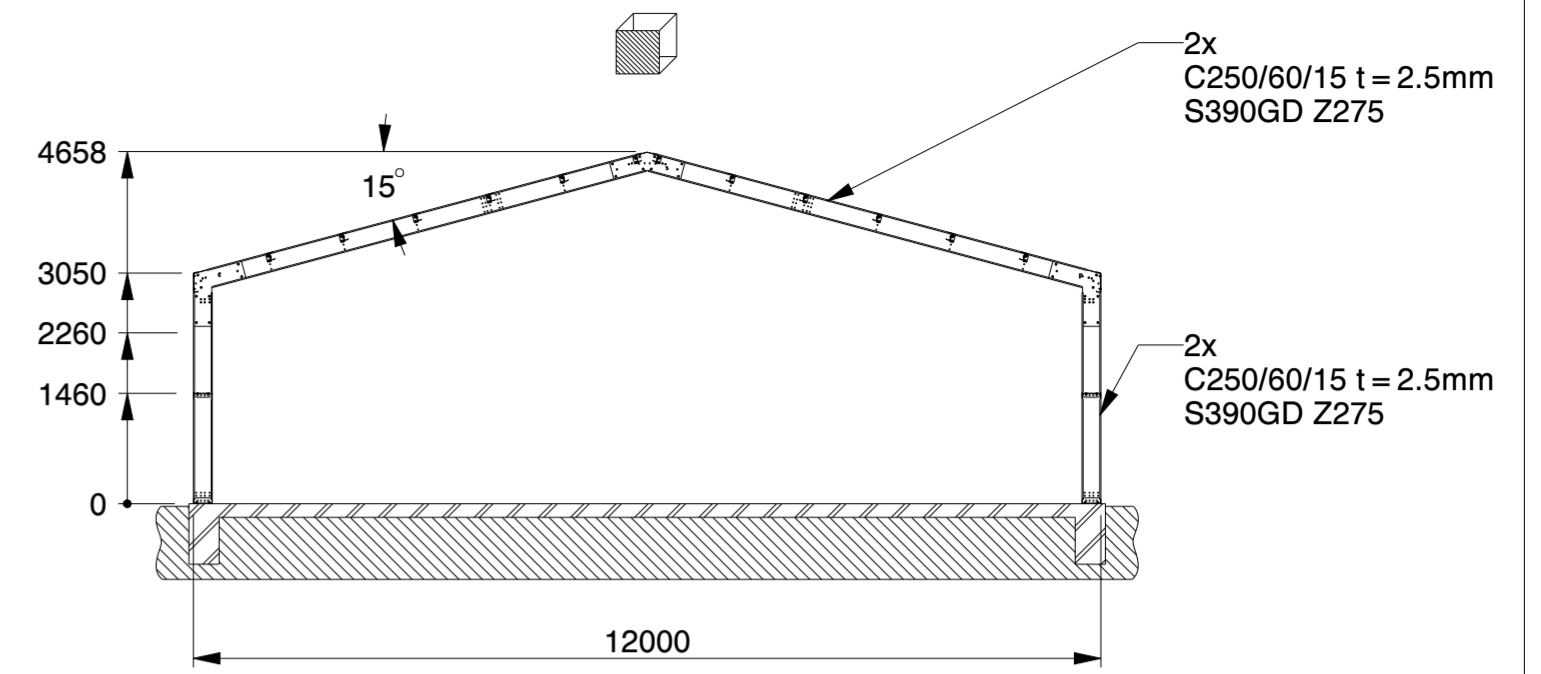
SECTION B-B
