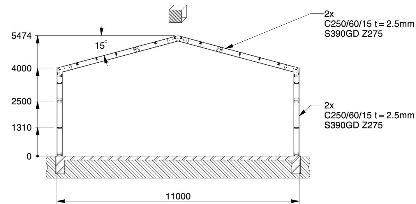
SECTION B-B
