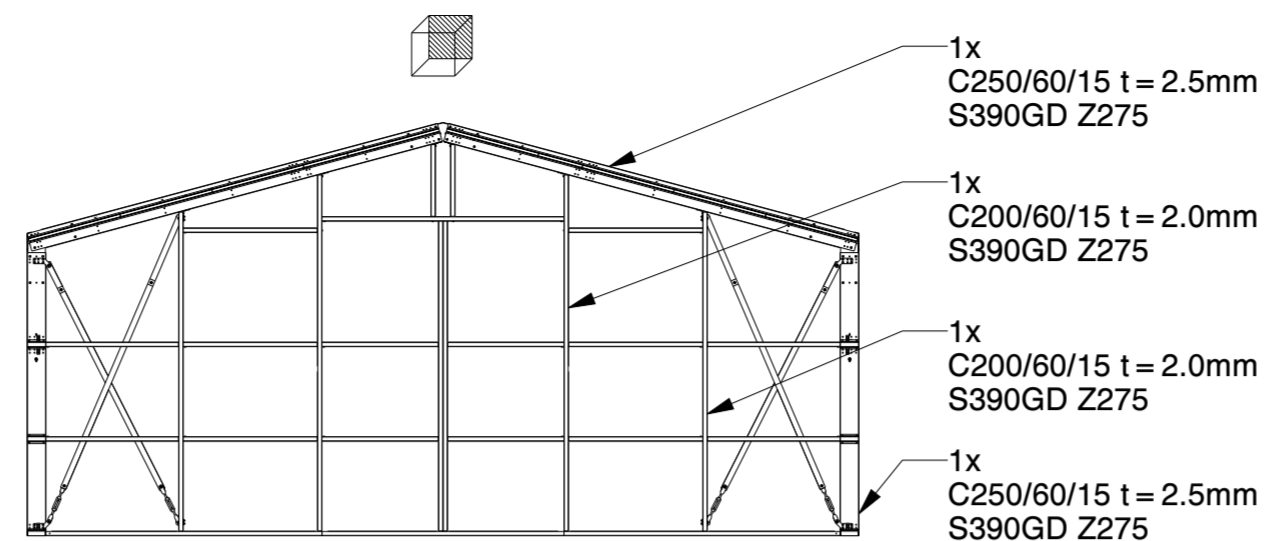
BACK WALL
