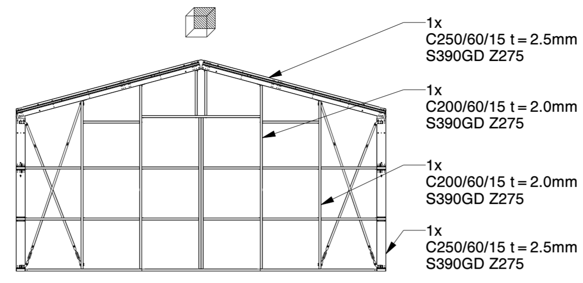
BACK WALL
