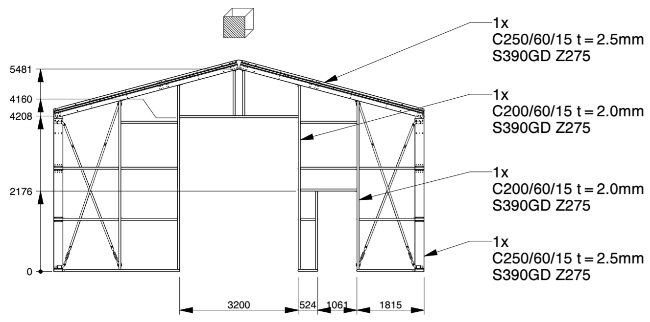
FRONT WALL
