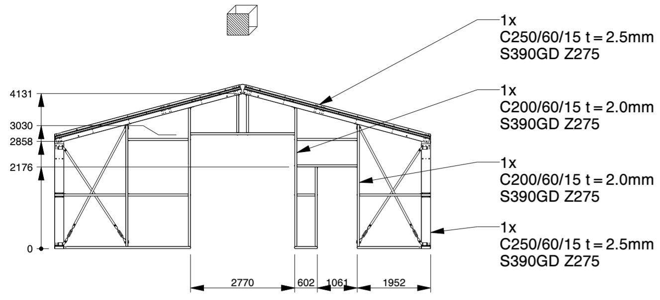
FRONT WALL
