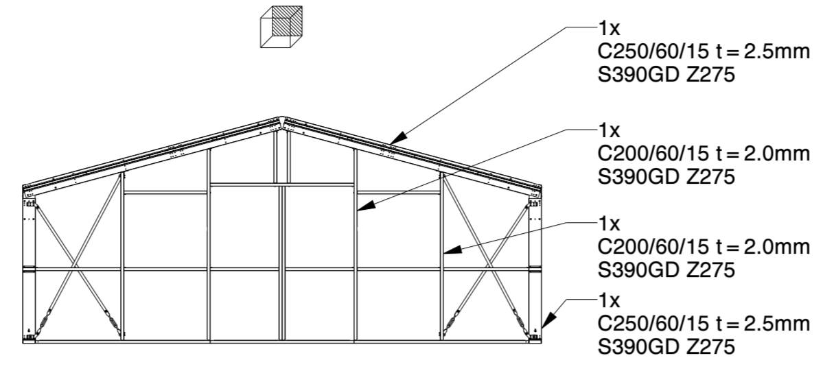
BACK WALL
