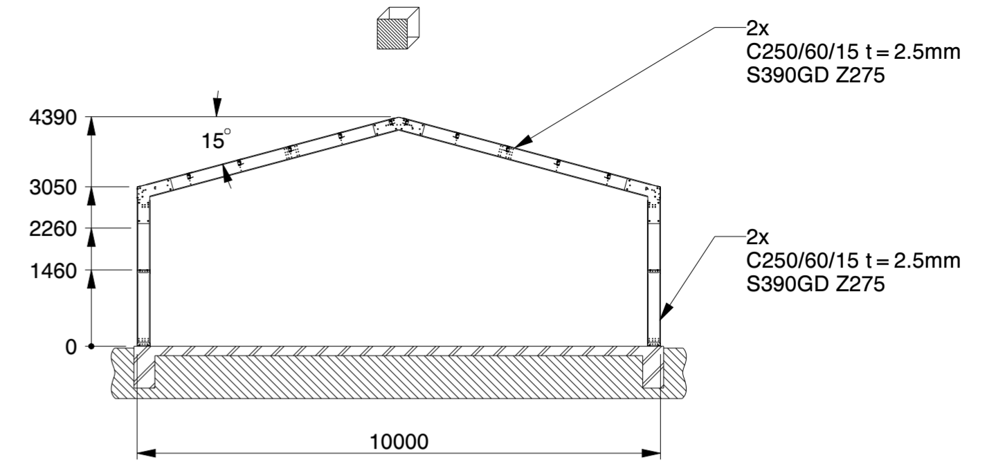
SECTION B-B
