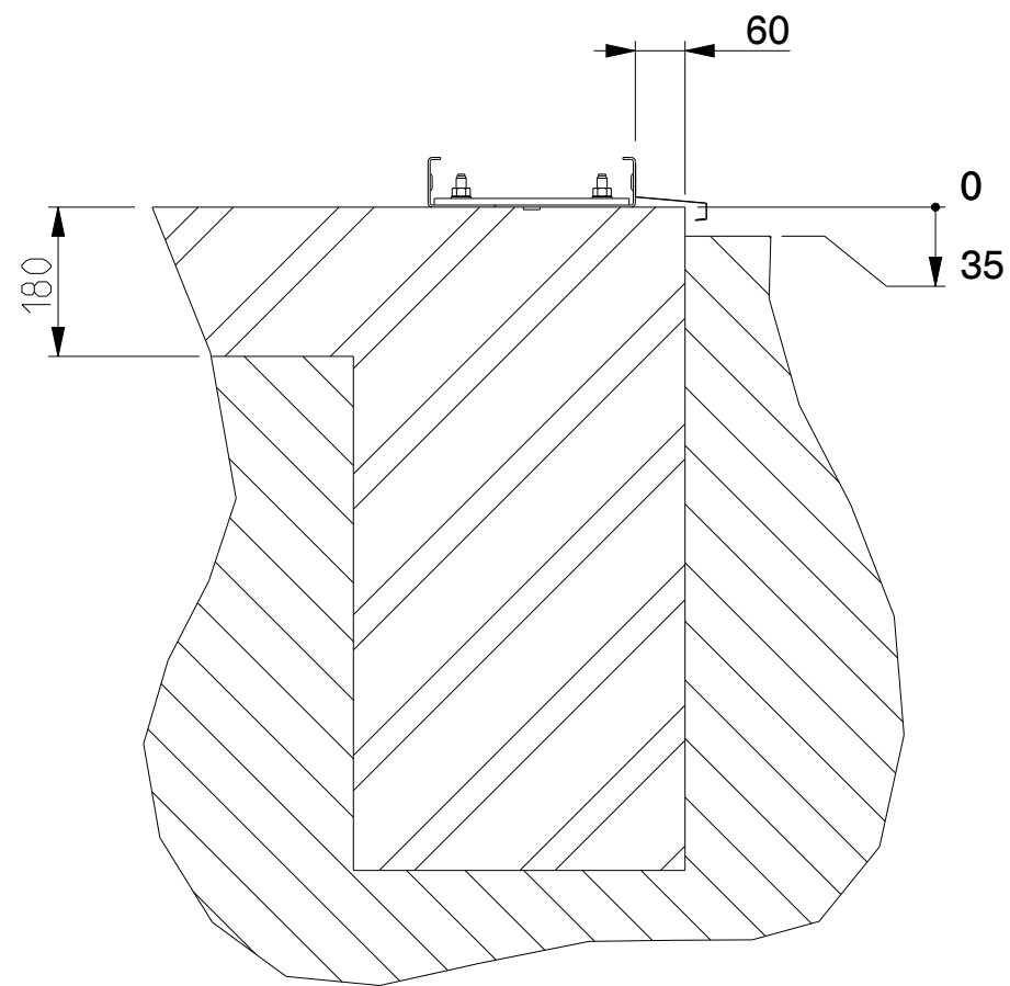
SECTION B-B
