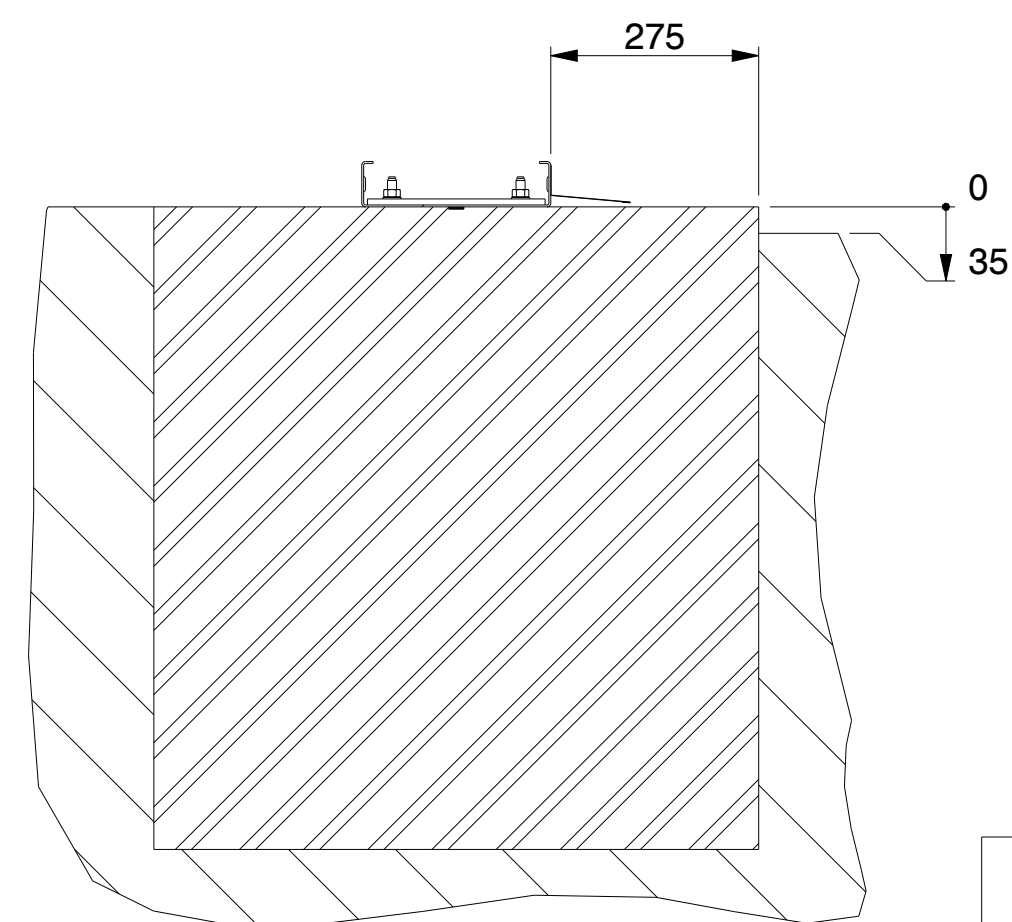
SECTION B-B
