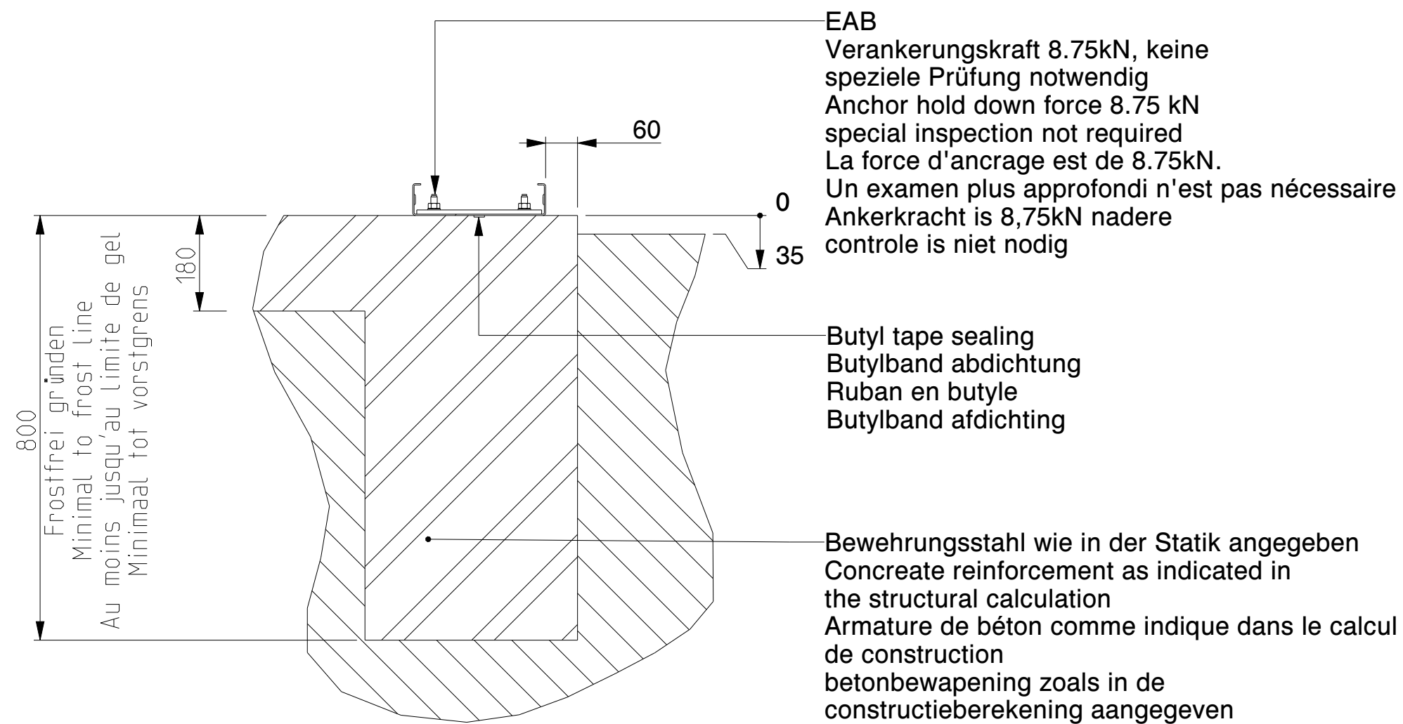
SECTION B-B
