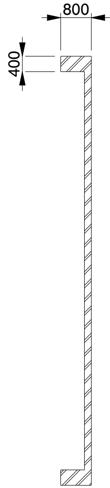
SECTION B-B
