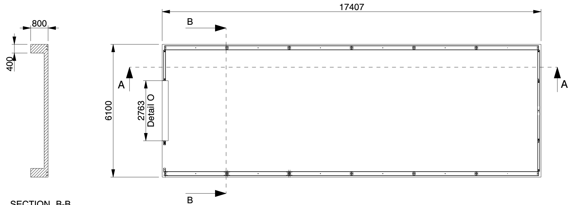
SECTION B-B
